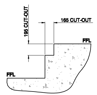
DETAIL 'A' DOOR OPERATOR CUT-OUT (CUT-OUT WIDTH = 1230) NOT SHOWN CLEARANCE SHALL BE REQUIRED IN UPPER THRESHOLD TO FACILITATE AUTOMATIC DOOR OPENER HOUSING
